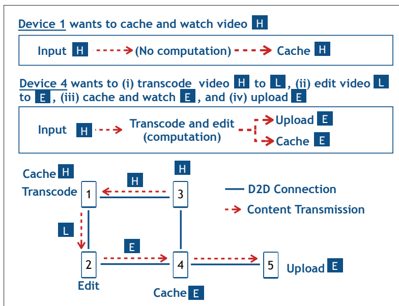
Figure 3. An example of the 3C framework.
